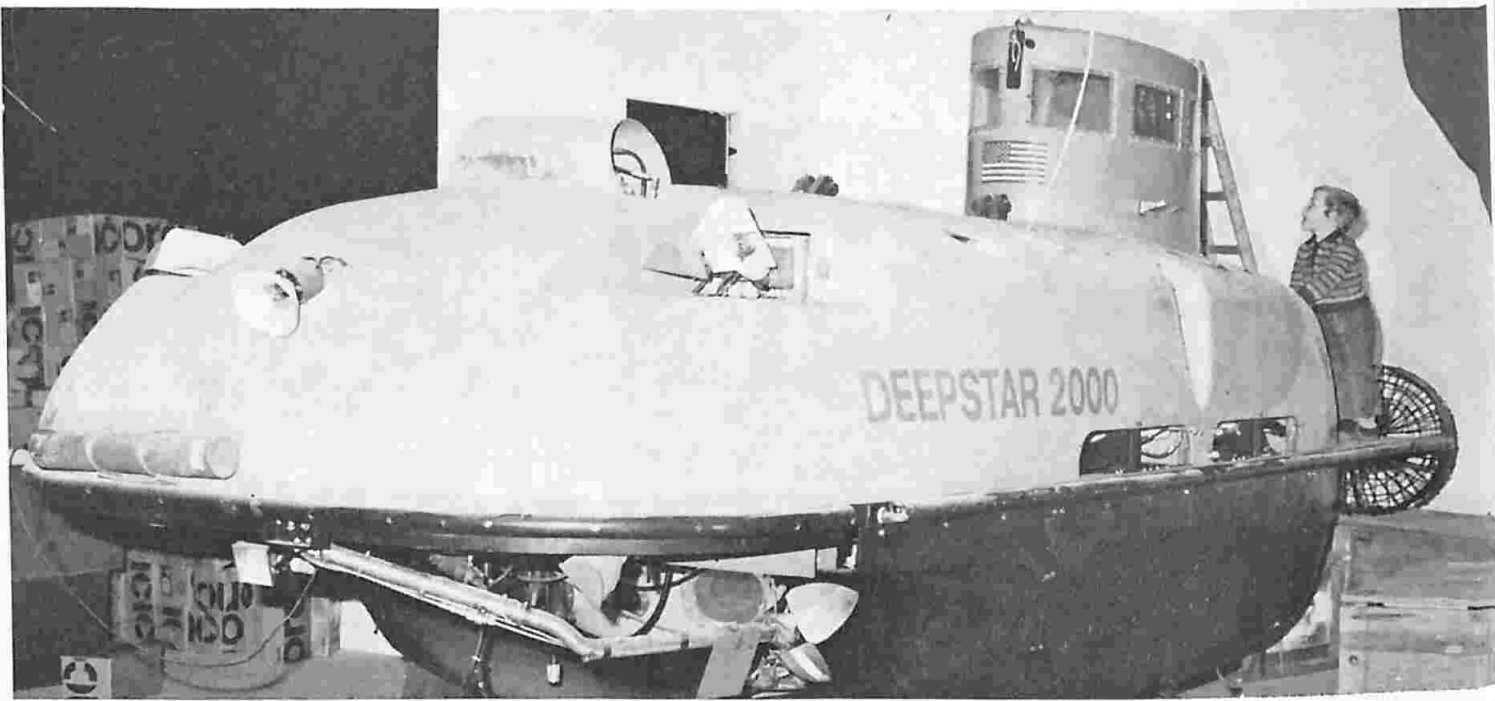
Deepstar 2000, a research submarine developed by the Westinghouse Electric Company, is one of the displays in the U. S. exhibit "Water Unlimited" at the German Industrial Exhibition Berlin 1973 at the Funkturm Exhibition Grounds through Nov. 11. The sub can dive to 600 meters with a crew of three. (Photo courtesy U. S. exhibit)
